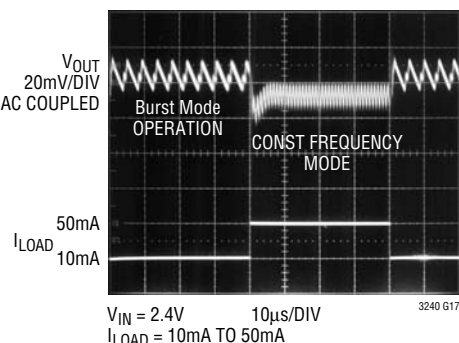
Load Transient Response (LTC3240-2.5)
