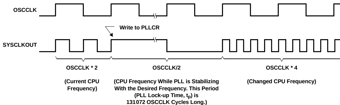
Figure 6-7. Example of Effect of Writing Into PLLCR Register
