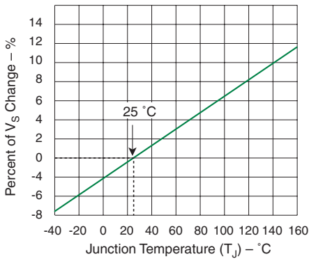
Normalized V_S Change versus Junction Temperature
