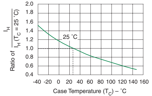
Normalized DC Holding Current versus Case Temperature
