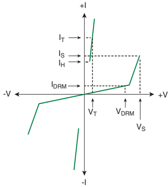
V-I Characteristics
