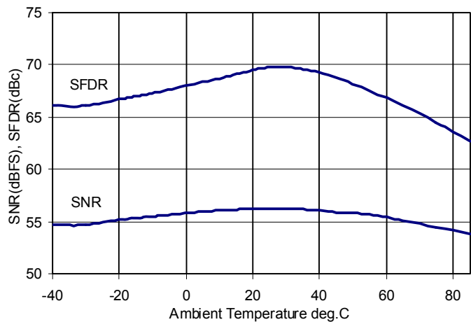
FIGURE 19. SNR vs TEMPERATURE
