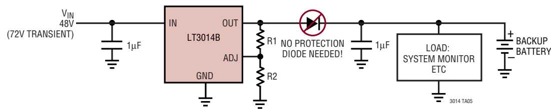
LT3014B Telecom Application
