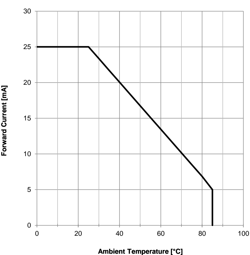
Derating Curve:
