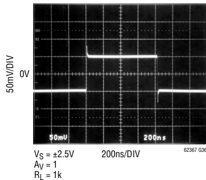
Small-Signal Response
