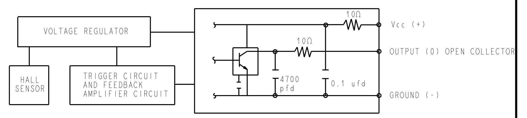
BLOCK DIAGRAM SHOWING CURRENT SINKING OUTPUT
