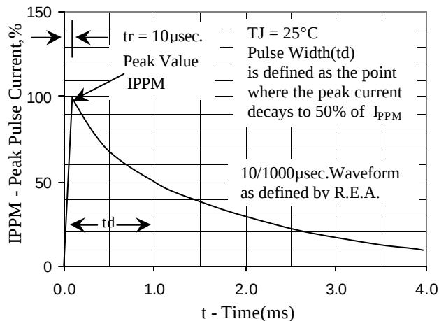
Fig.3 - Pulse Waveform
