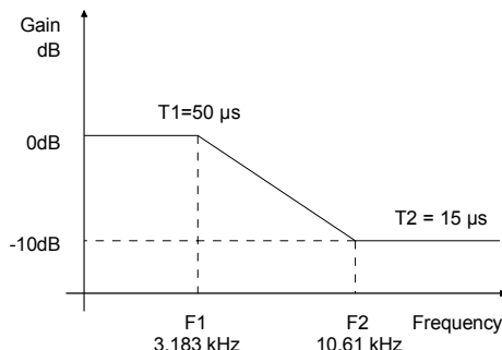
Figure 14. De-Emphasis Curve
