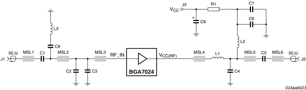
See Table 11 for a list of components. PCB specification: Rogers RO4003C; height = 0.508 mm; \epsilon_r = 3.38 ; copper thickness = 35 \mu\text{m} .
