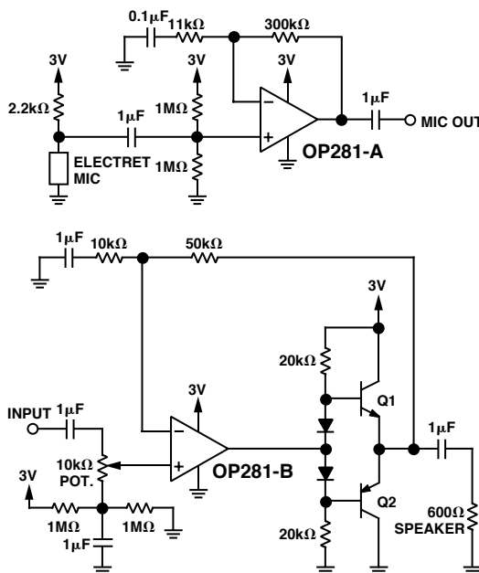
Figure 10. Two-Way Amplifier in a Battery-Powered Telephone Headset
