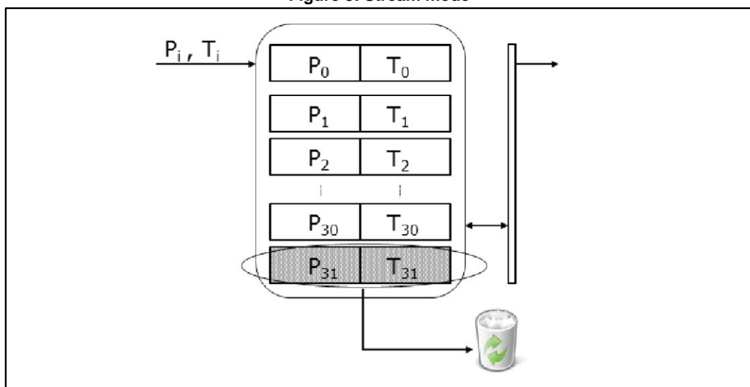
Figure 8: Stream mode
