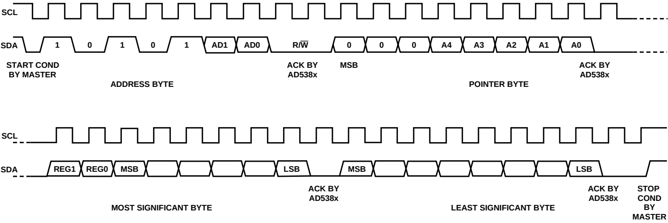
Figure 31. 4-Byte AD5382, I 2 C Write Operation
