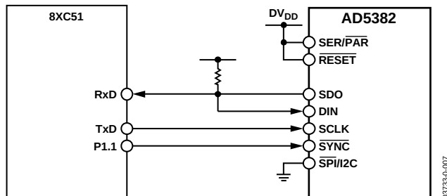
Figure 37. AD5382-to-8051 Interface
