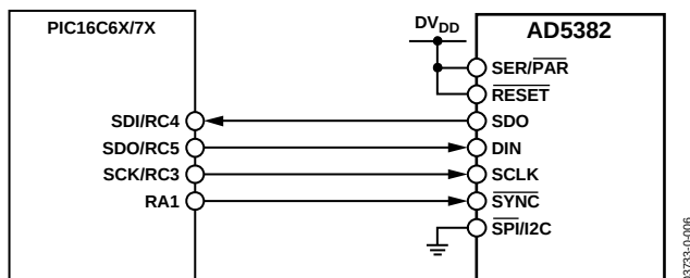
Figure 36. AD5382-to-PIC16C6x/7x Interface
