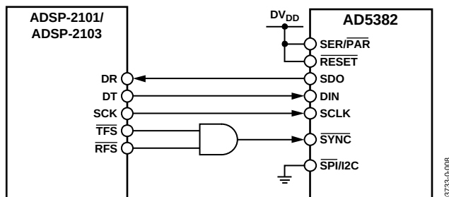
Figure 38. AD5382-to-ADSP-2101/ADSP-2103 Interface
