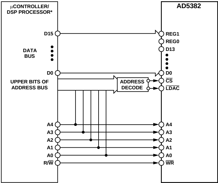
Figure 35. AD5382-to-Parallel Interface
