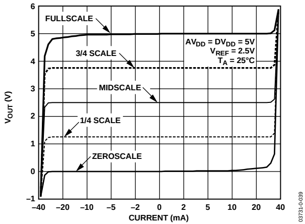
Figure 21. AD5382-5 Output Amplifier Source and Sink Capability
