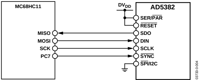
Figure 34. AD5382-to-MC68HC11 Interface
