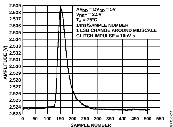
Figure 10. AD5382-5 Glitch Impulse
