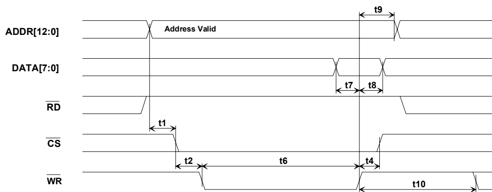
Figure 11-10 Intel Bus Write Timing (HWMODE = 0, MODEC = 00)
