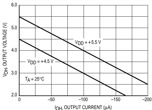
Figure 20. ST1, V_{OH} versus I_{OH}
