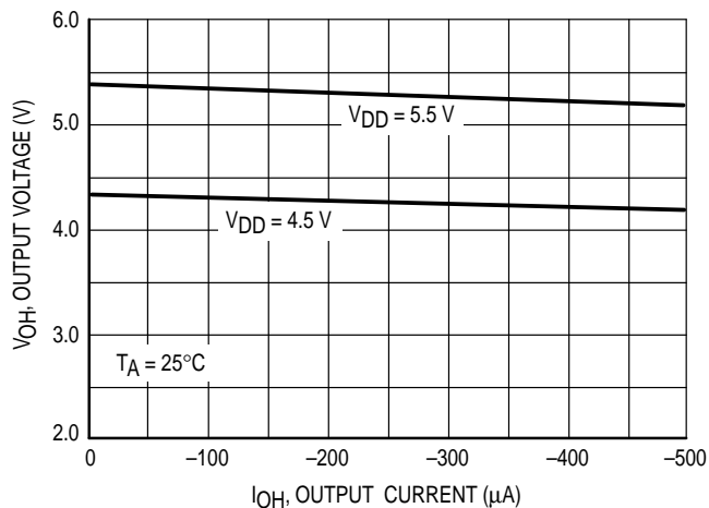
Figure 22. ST2, V_{OH} versus I_{OH}
