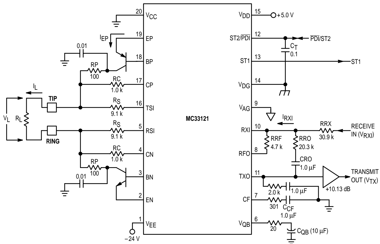
Figure 1. Test Circuit
