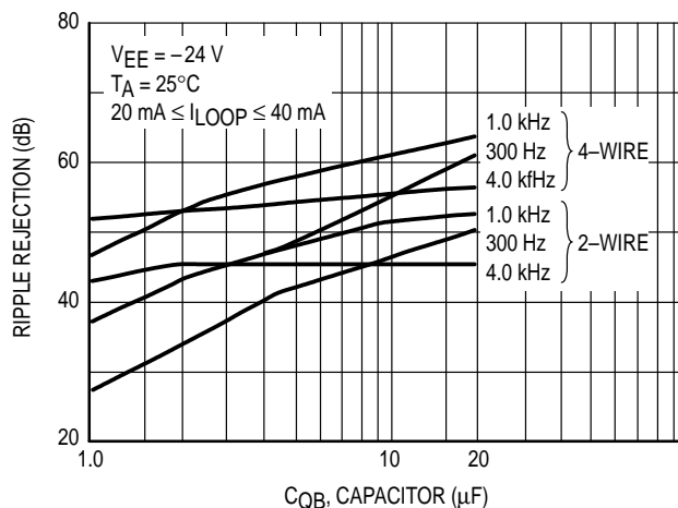
Figure 18. V_{EE} Ripple Rejection versus Frequency and C_{QB}
