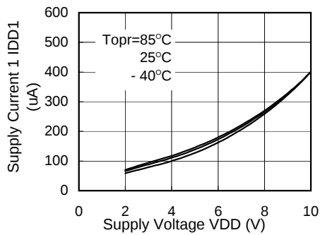
(6) Stand-by Current vs. Supply Voltage
