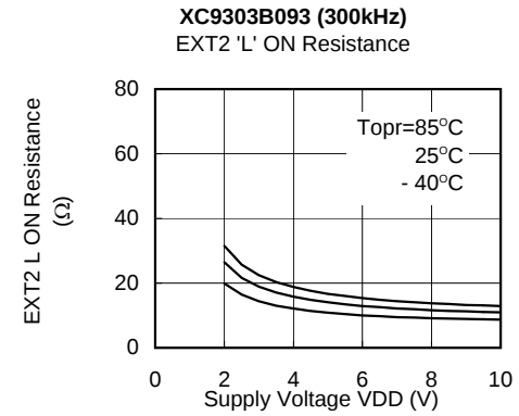
(15) EXT2 Low ON Resistance vs. Supply Voltage
