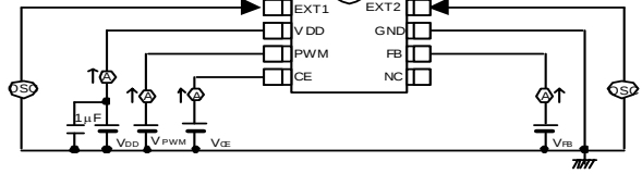
Circuit 4
