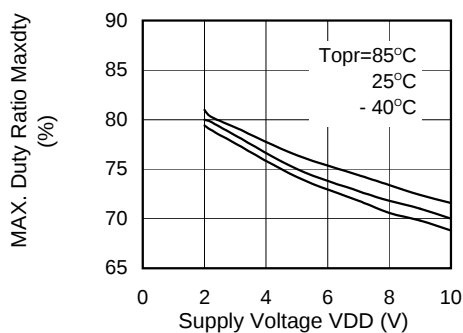
(10) Maximum Duty Ratio vs. Supply Voltage
