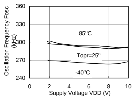
(11) Oscillation Frequency vs. Supply Voltage
