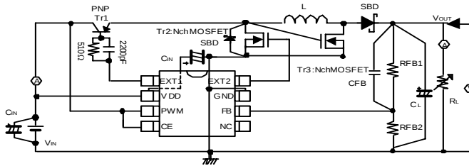
Circuit 3
