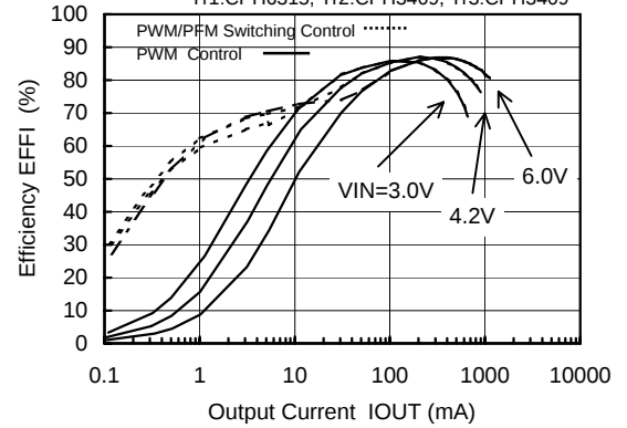
FOSC=300kHz, VOUT=5.0V
