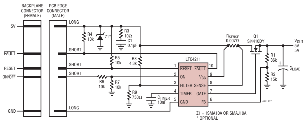
Figure 27. LTC4211MS High Side Overvoltage Protection Implementation (In Normal Mode, SLOW COMP Is Disabled. In Soft-Start Cycle, I_{\text{SOFTSTART}} Is Still 50\text{mV}/R_{\text{SENSE}} )
