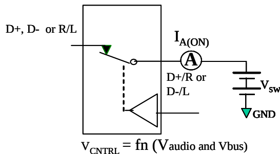
Figure 12. On Leakage
