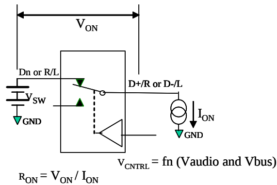
Figure 10. On Resistance
