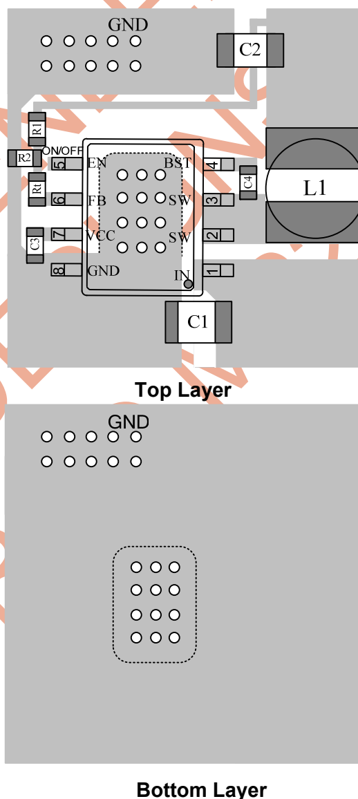
Figure 4—PCB Layout
