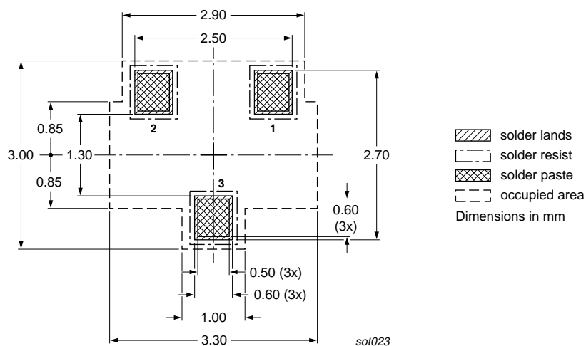
Fig 7. Reflow soldering footprint SOT23 (TO-236AB)
