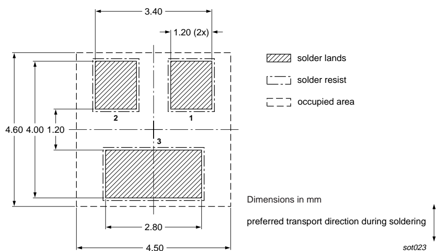
Fig 8. Wave soldering footprint SOT23 (TO-236AB)
