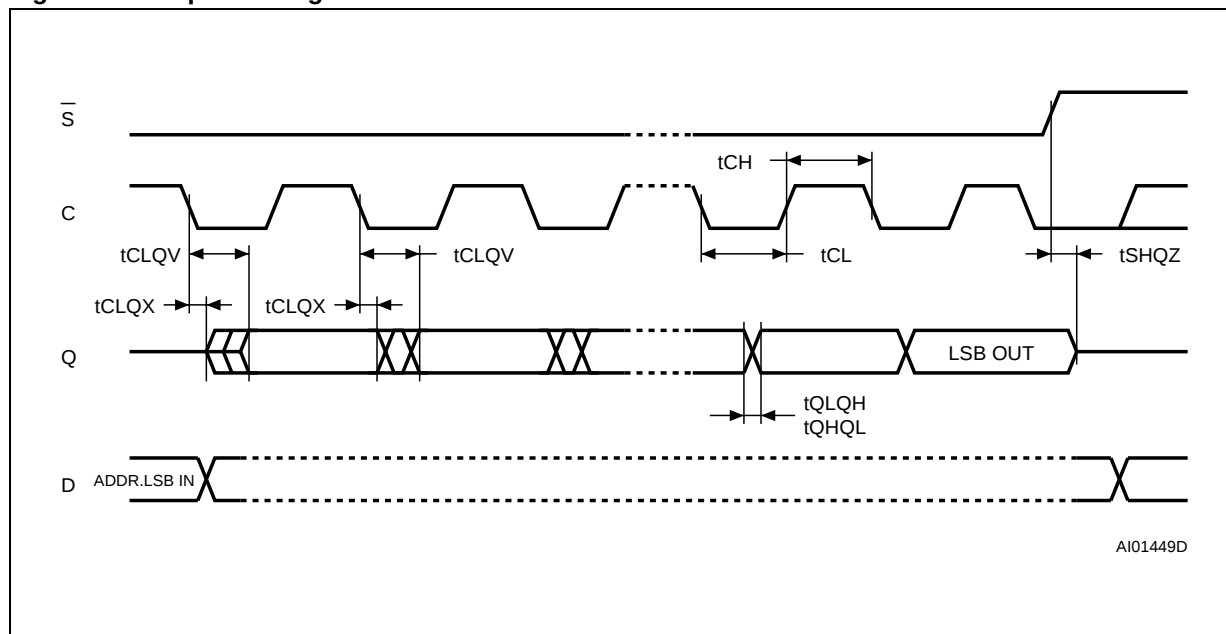
Figure 24. Output Timing
