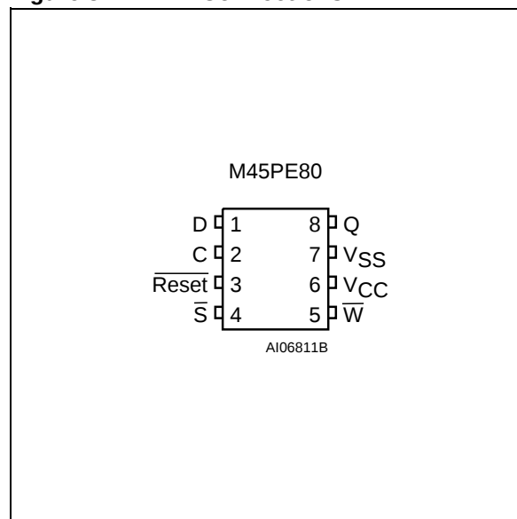
Figure 3. VDFPN Connections
