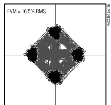
COMPOSITE EVM W-CDMA: PCCPCH + SCH
