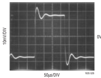
Small-Signal Transient Response V_S = \pm 5V
