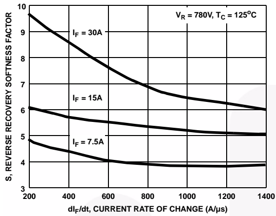
Figure 7. Reverse Recovery Softness Factor vs dI F /dt
