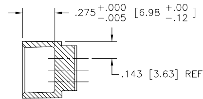
SECTION X-X
