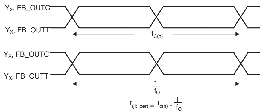
Figure 6. Period Jitter
