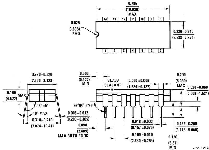
14-Lead Ceramic Dual-In-Line Package (J) Order Number DM54LS27J Package Number J14A
