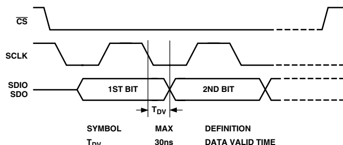
Figure 53. Timing Diagram for Read from AD9852
