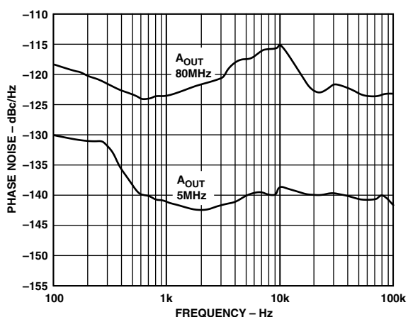
Figure 18b. Residual Phase Noise, 30 MHz REFCLK with REFCLK Multiplier = 10×
