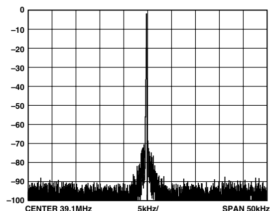
Figure 17. Narrowband SFDR, 39.1 MHz, 50 kHz BW, 20 MHz REFCLK with REFCLK Multiplier = 10×
