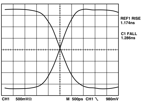
Figure 22. Comparator Rise/Fall Times
