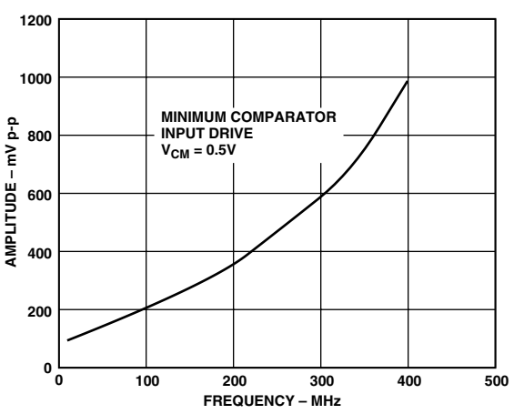
Figure 23. Comparator Toggle Voltage Requirement
