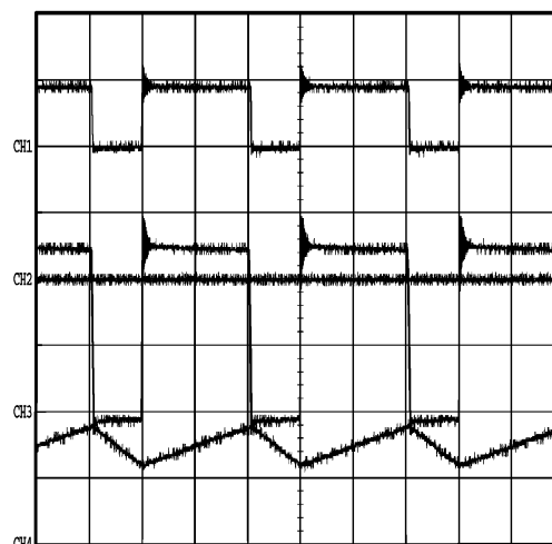
Figure 6. Illustrating Buck Operation
