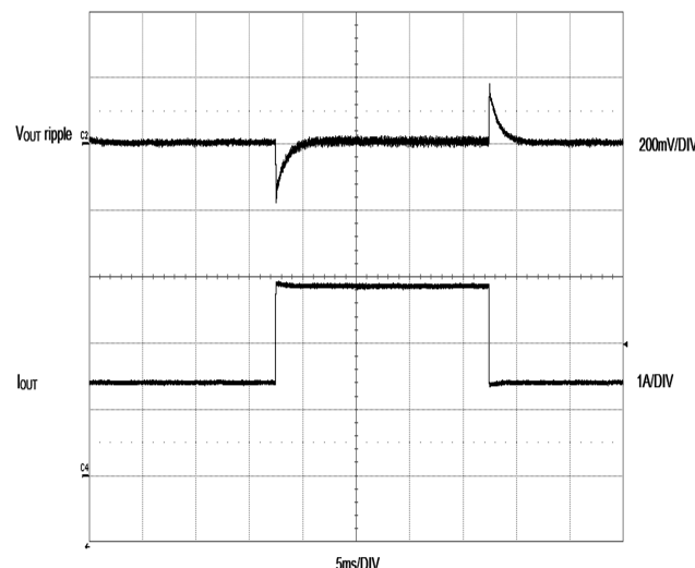
Figure 8. Buck-Boost Mode Transient Response
