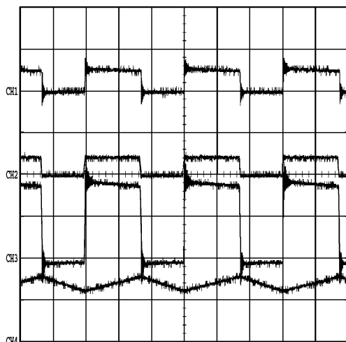
Figure 5. Illustrating Buck-Boost Operation
