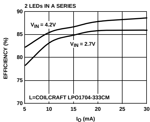
FIGURE 5B. EFFICIENCY vs I_0
