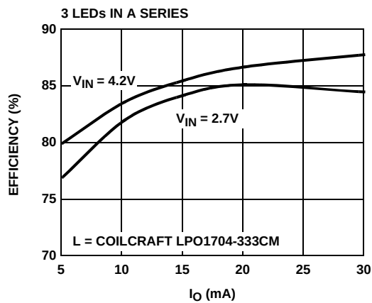
FIGURE 6B. EFFICIENCY vs I_0
