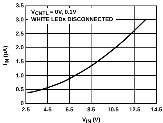
FIGURE 2. QUIESCENT CURRENT
