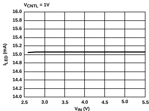
FIGURE 4. I_{LED} vs V_{IN}
