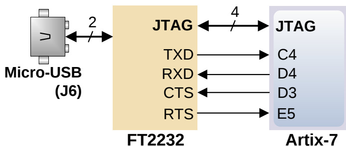
Figure 6. Nexys4 FT2232HQ connections
