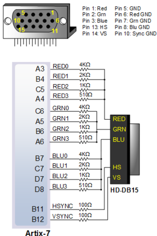
Figure 11. Nexys4 VGA Interface
