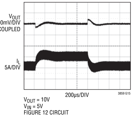
Load Step (Boost) Forced Continuous Mode
