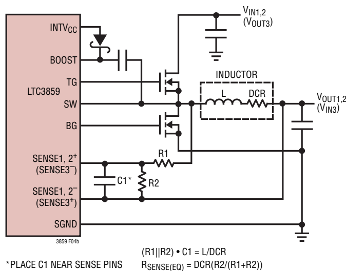
4b. Using the Inductor DCR to Sense Current
