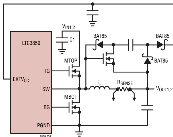
Figure 9. Capacitive Charge Pump for EXT CC
