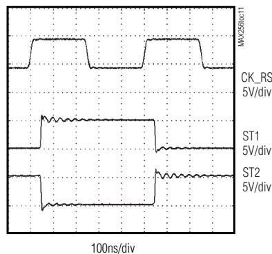
OPERATION WITH EXTERNAL 2MHz CLOCK
