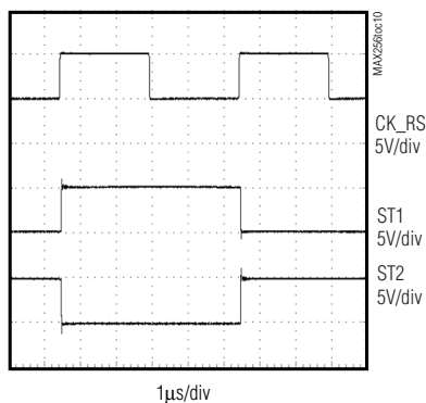
OPERATION AT 100kHz
