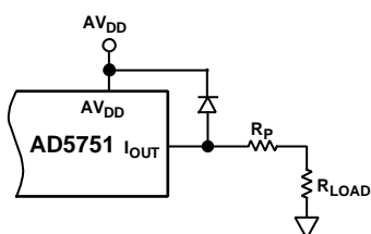
Figure 15. Output Transient Voltage Protection
