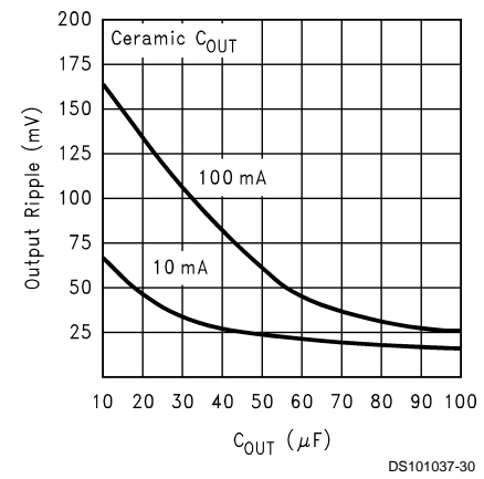
V_{OUT} Ripple vs. C_{OUT}
