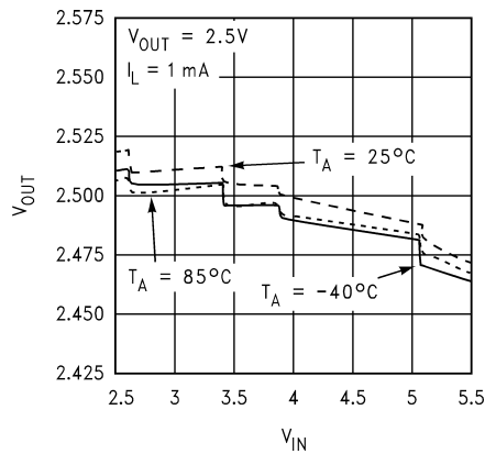
V_{\text{OUT}} vs. V_{\text{IN}}
