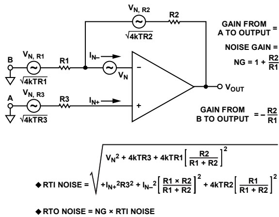
Figure 50. Op Amp Noise Analysis Model
