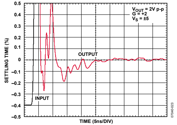
Figure 23. Short-Term Settling Time (LFCSP)
