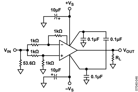
Figure 45. Common-Mode Rejection
