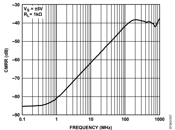
Figure 37. Common-Mode Rejection Ratio (CMRR) vs. Frequency
