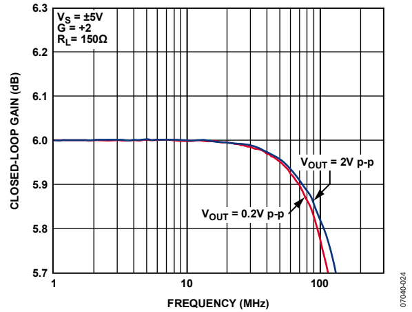
Figure 24. 0.1 dB Flatness vs. Frequency for Various Output Voltages (LFCSP)
