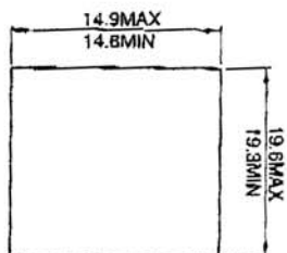
Single Panel - Latch Clearance Panel Thickness 0.062
