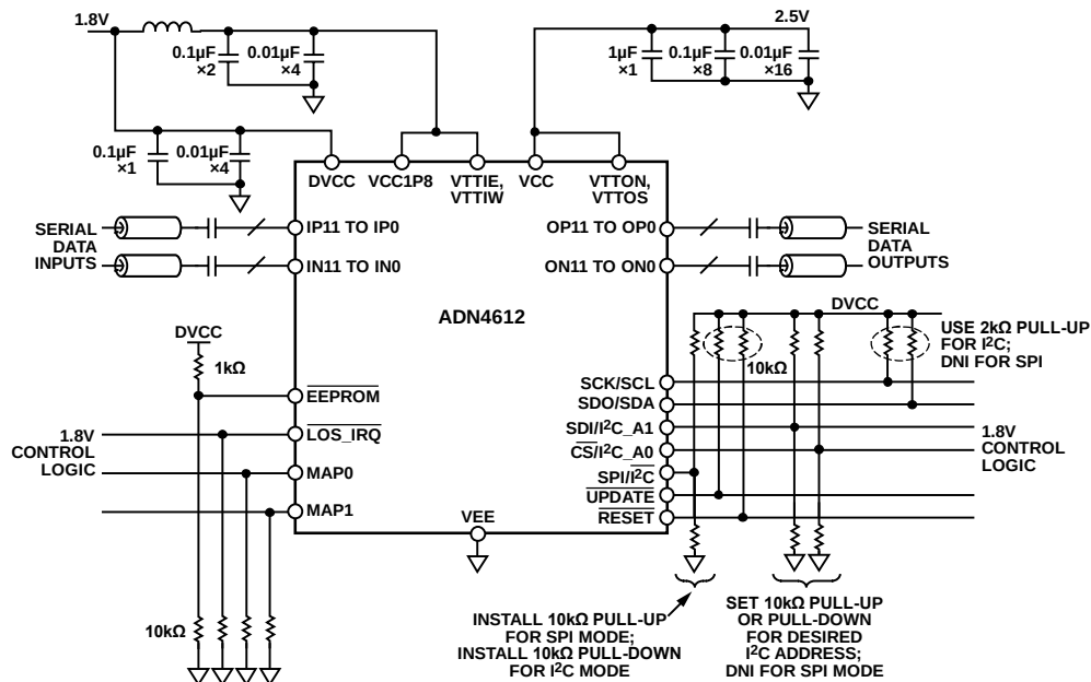
Figure 73. Applications Circuit
