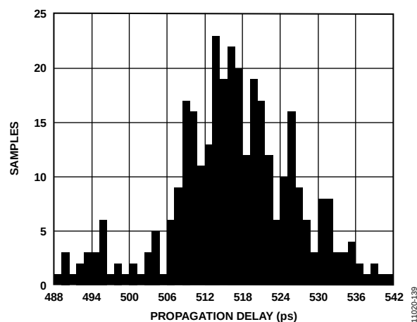
Figure 26. Propagation Delay Histogram
