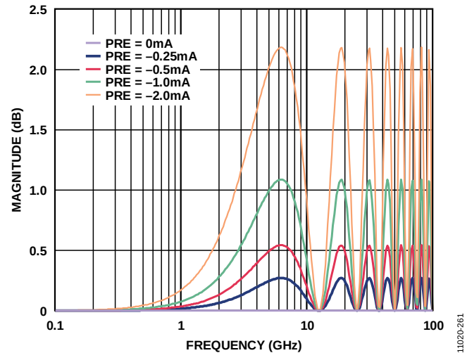
Figure 57. Transmit FIR Response (Precursor Only)
