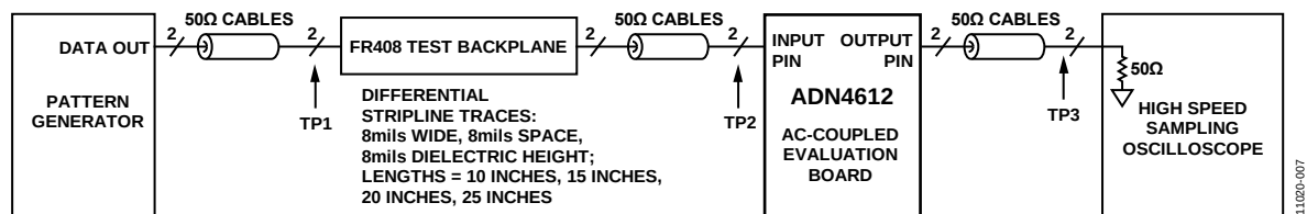
Figure 48. Equalization Test Circuit
