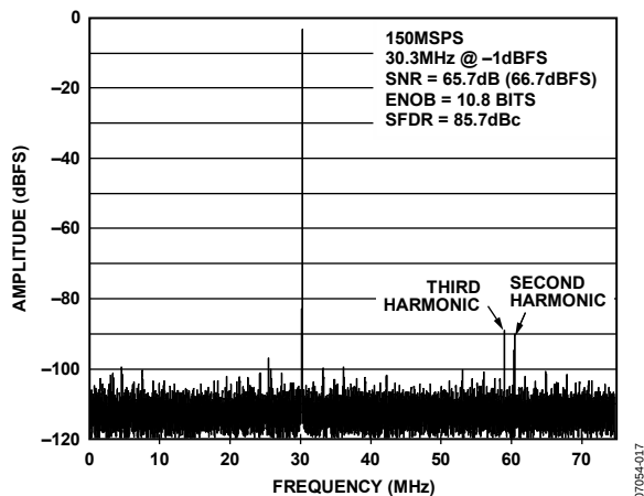
Figure 17. AD9627-11-150 Single-Tone FFT with f_{IN} = 30.3 MHz
