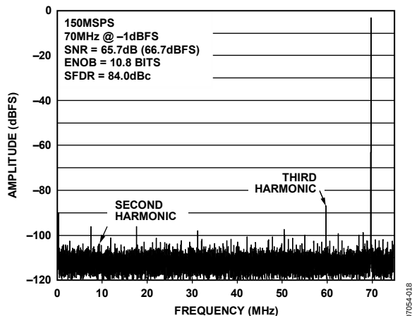
Figure 18. AD9627-11-150 Single-Tone FFT with f_{IN} = 70 MHz
