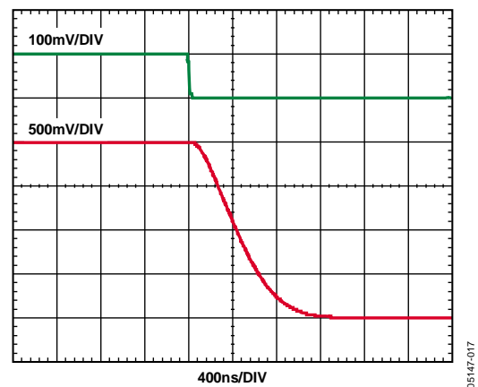
Figure 9. Fall Time
