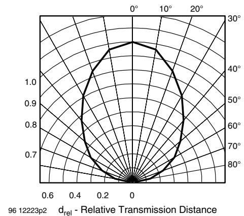
Fig. 4 - Horizontal Directivity
