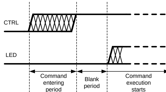
Figure 8. Single-Wire Interface
