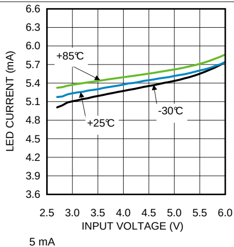
Figure 4. LED Current vs Input Voltage
