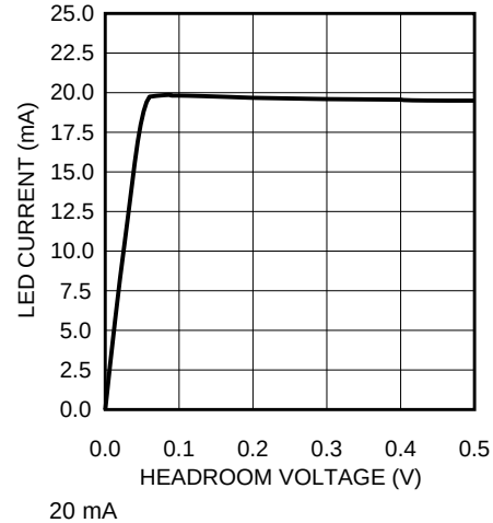
Figure 7. I_{OUT} vs Headroom Voltage
