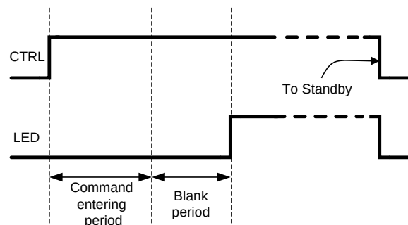
Figure 10. Follow Mode
