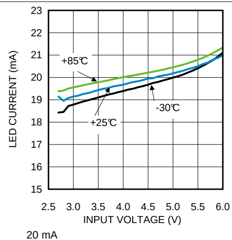
Figure 5. LED Current vs Input Voltage
