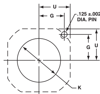
mounting dimensions
