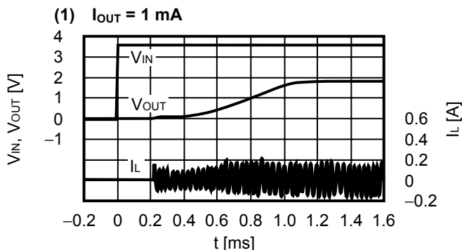
3.1 Powering ON ( V_{OUT} = 1.8 V, V_{IN} = 0 V \rightarrow 3.6 V, T_a = 25^\circ\text{C} )
