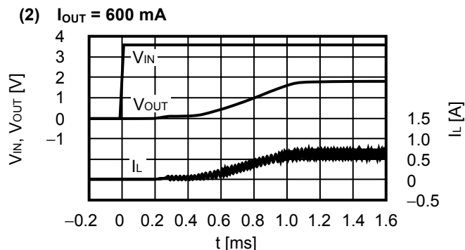
3.2 Shutdown pin response ( V_{OUT} = 1.8 V, V_{IN} = 3.6 V, V_{ON/OFF} = 0 V \rightarrow 3.6 V, T_a = 25^\circ\text{C} )
