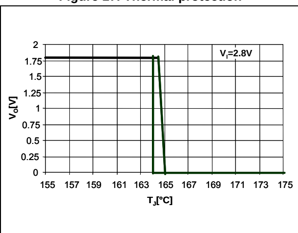
Figure 17. Thermal protection
