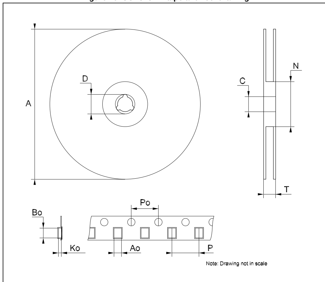
Figure 19. SOT323-xL tape and reel drawing
