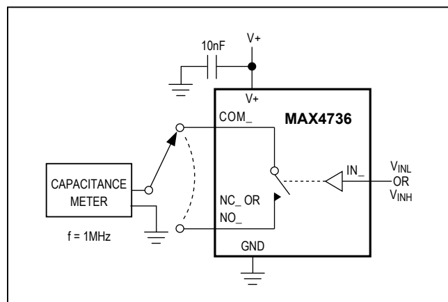
Figure 4. Channel Off/On-Capacitance
