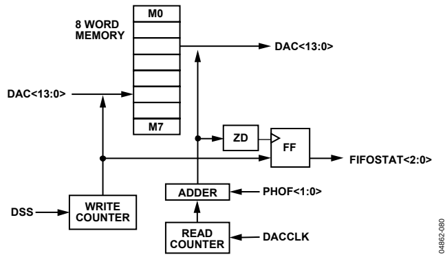
Figure 82. Sync Logic Block Diagram
