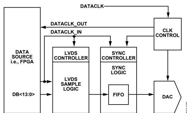
Figure 77. Data Controllers
