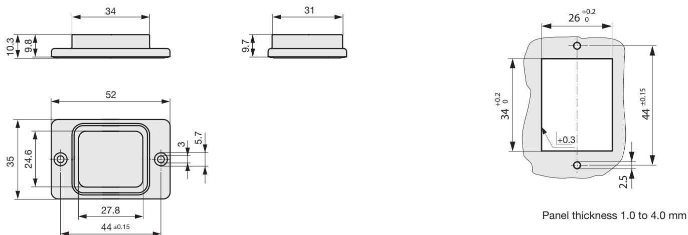
CZZ21, Screw-on Collar with Cover, IP65 Part. No. 4435.0053
