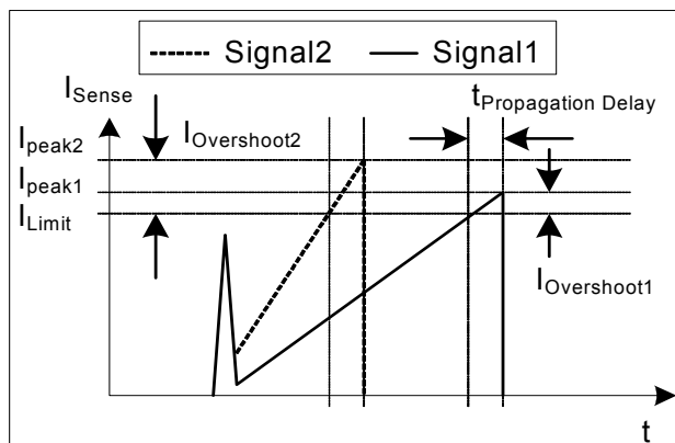
Figure 19 Current Limiting
