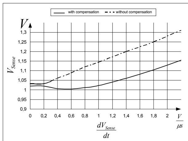
Figure 20 Overcurrent Shutdown
